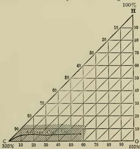
FIG. 12.—Trilinear Coordinates on an Isosceles Triangle.
